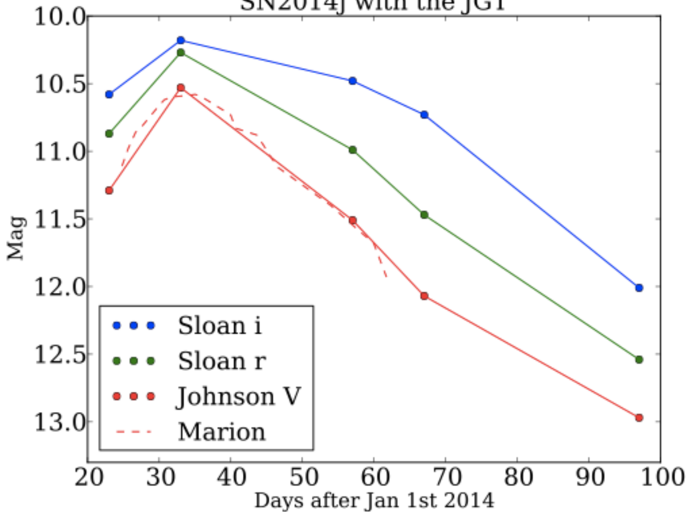
SN2014j with the JGT
